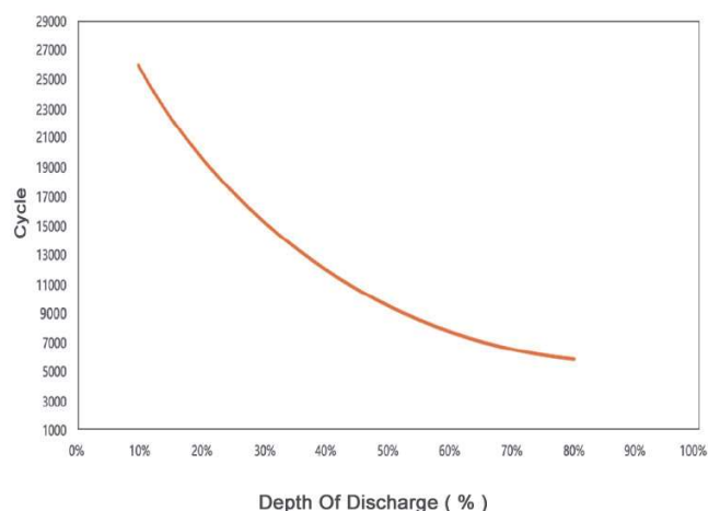
Cycle Times vs. DOD in HESS Scenario at 35°C
