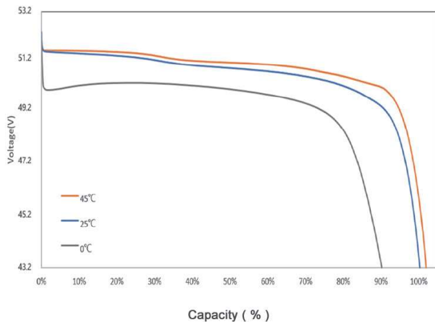
Discharge Curve @0.2C, Different temp
